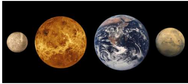
Figure 6.2: Images of the four innermost terrestrial planets
